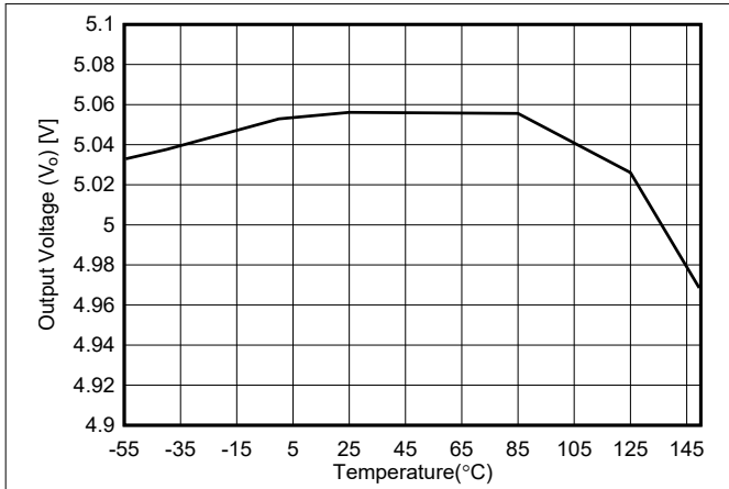
Figure 6-1. V_O vs Temperature for New Chip
