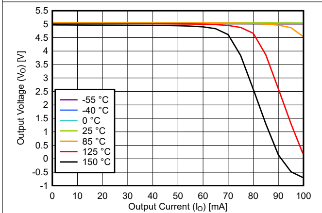
Figure 6-3. Load Regulation for Legacy Chip
