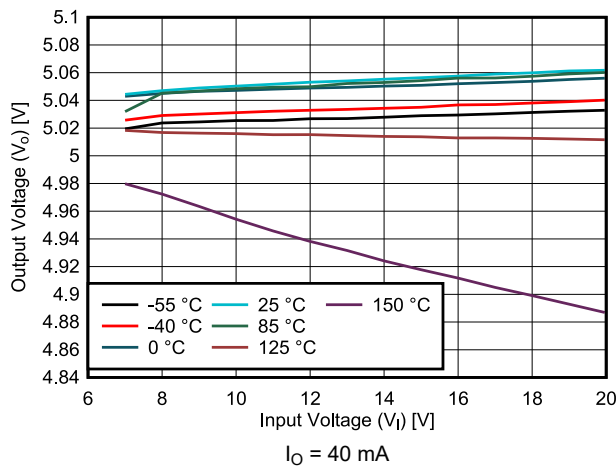
Figure 6-9. Line Regulation at I_O = 40\text{ mA} for New Chip
